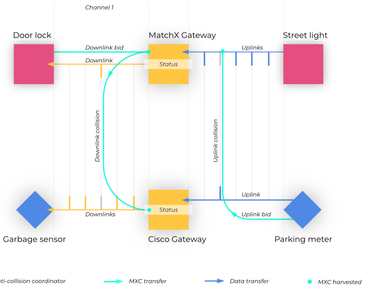
Figure 5: MXProtocol Anti-Collision Coordinator
